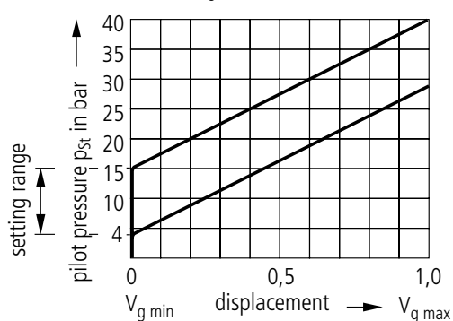
Characteristic curve: hydraulic stroke limiter, H2
